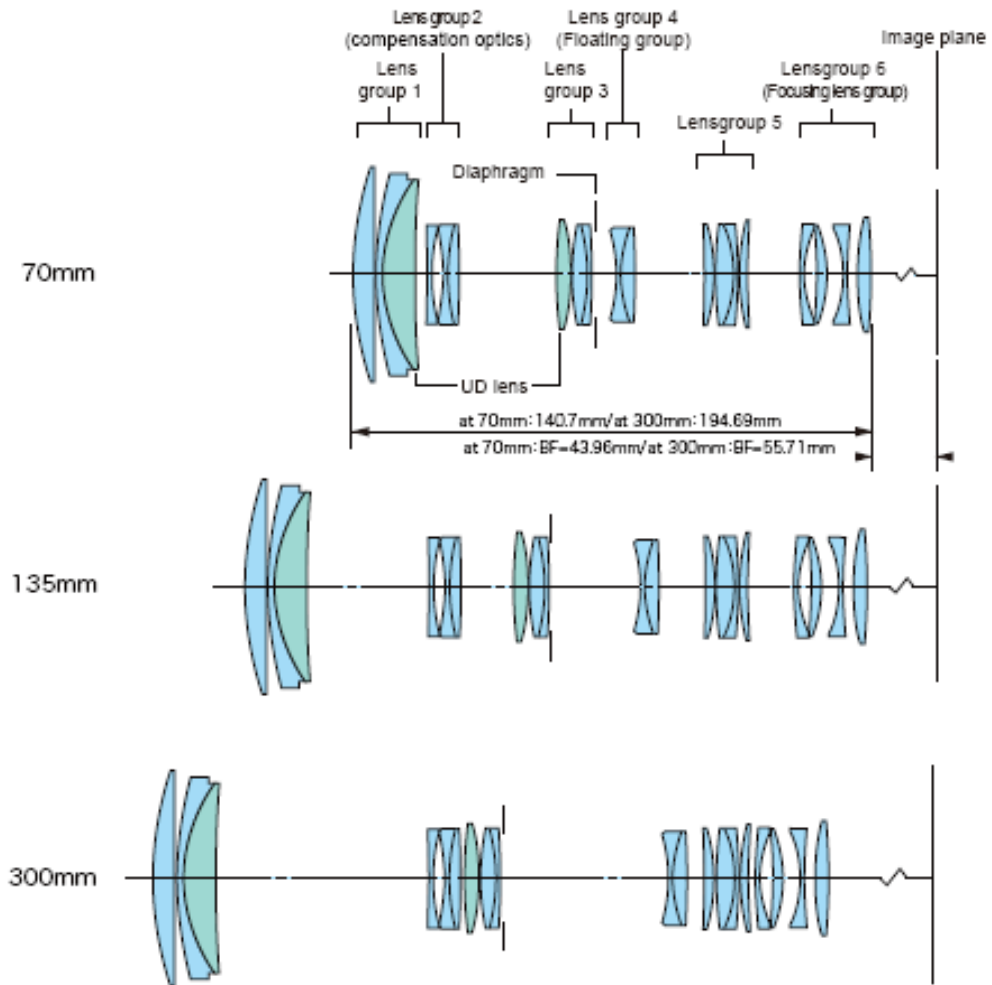
EF70-300mm f/4-5.6L IS USM lens movement during zooming.
